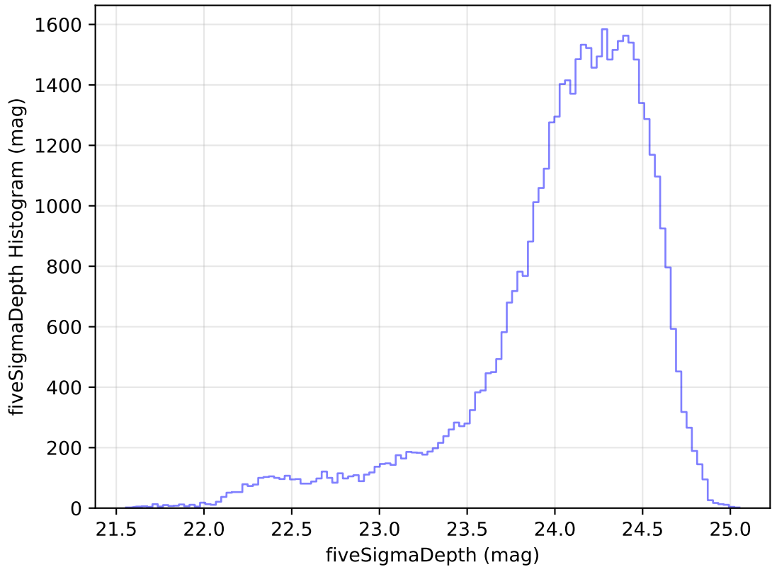
internal_u_expt38_nscale1.2v3.4_10yrs Yr 1 r band: fiveSigmaDepth Histogram
