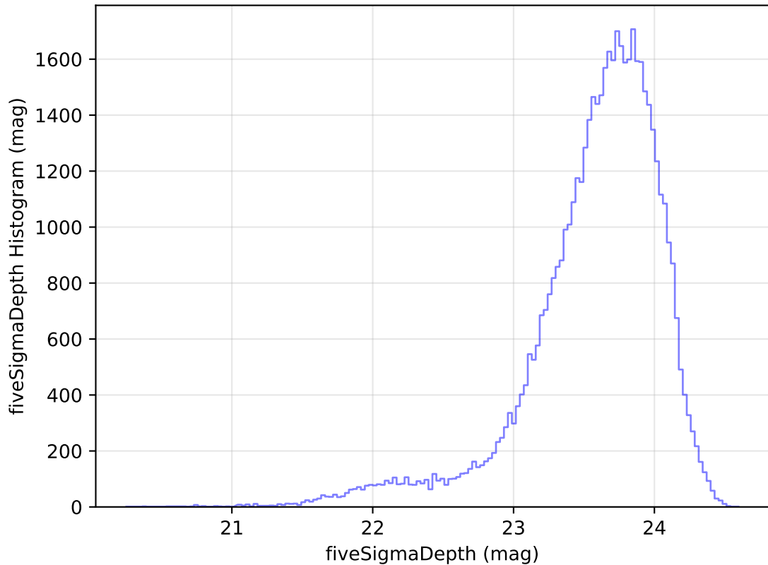
internal_u_expt38_nscale1.2v3.4_10yrs Yr 1 i band: fiveSigmaDepth Histogram
