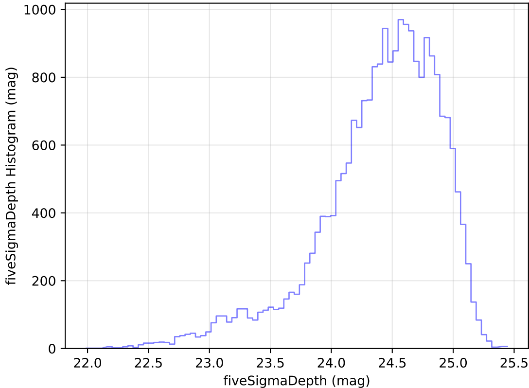
internal_u_expt38_nscale1.2v3.4_10yrs Yr 1 g band: fiveSigmaDepth Histogram
