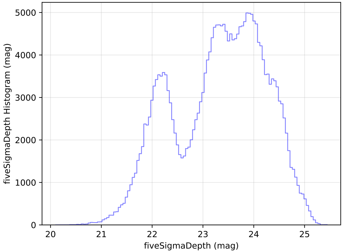
internal_u_expt38_nscale1.2v3.4_10yrs Yr 1 all bands: fiveSigmaDepth Histogram
