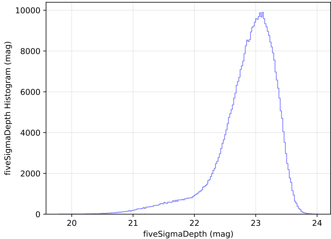
internal_u_expt38_nscale1.2v3.4_10yrs WFD z band: fiveSigmaDepth Histogram
