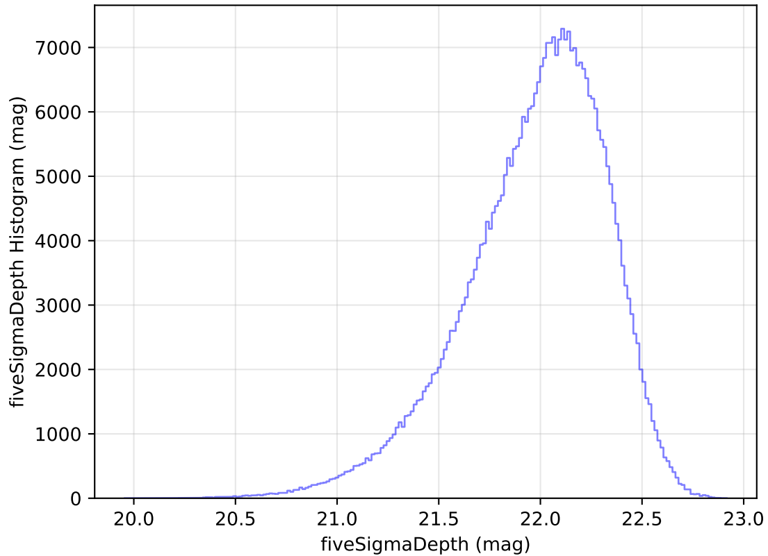
internal_u_expt38_nscale1.2v3.4_10yrs WFD y band: fiveSigmaDepth Histogram
