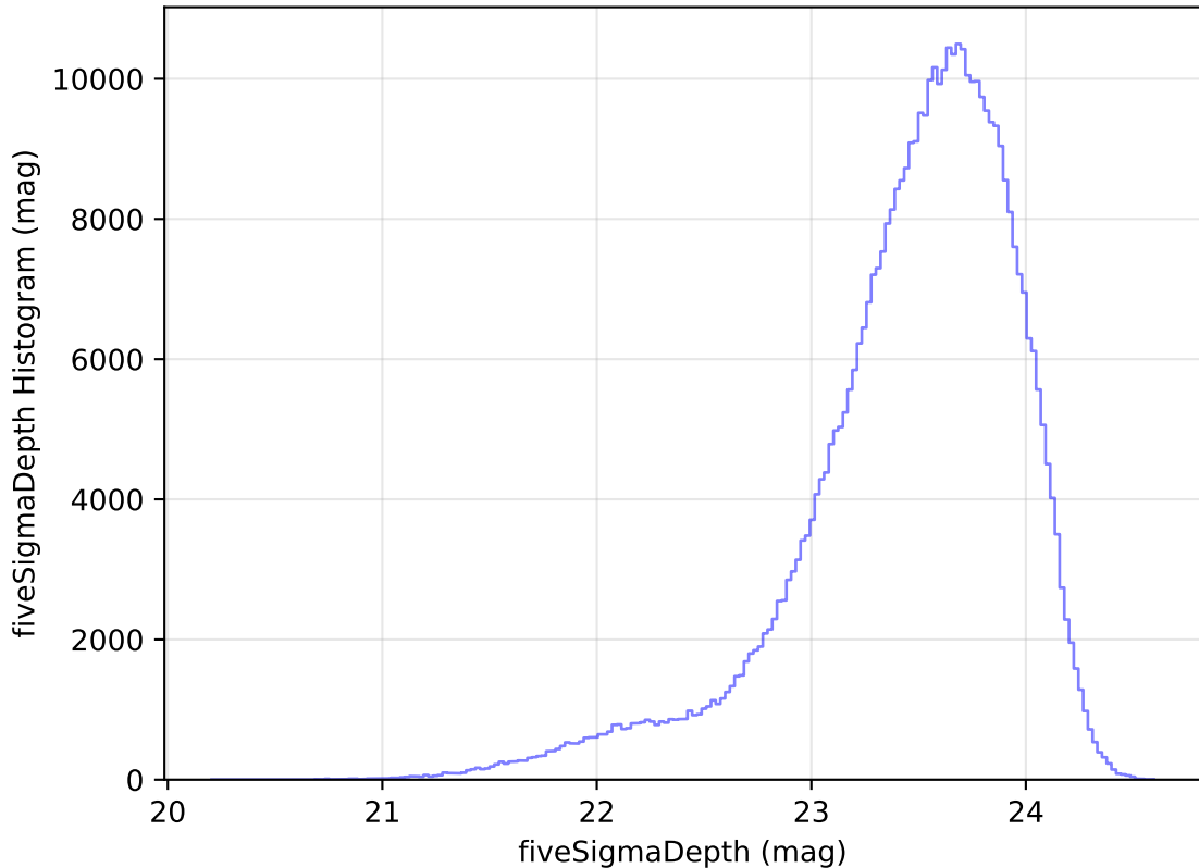
internal_u_expt38_nscale1.2v3.4_10yrs WFD i band: fiveSigmaDepth Histogram
