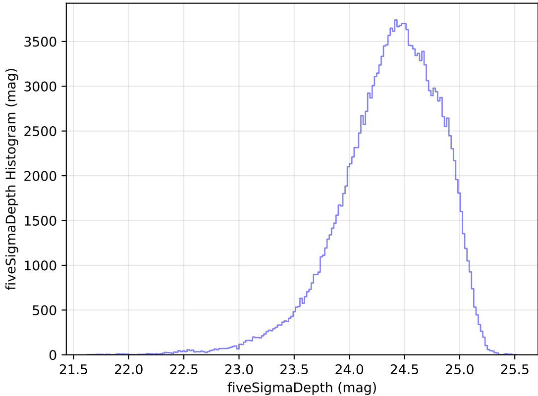
internal_u_expt38_nscale1.2v3.4_10yrs WFD g band: fiveSigmaDepth Histogram
