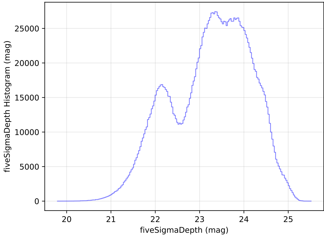
internal_u_expt38_nscale1.2v3.4_10yrs WFD all bands: fiveSigmaDepth Histogram
