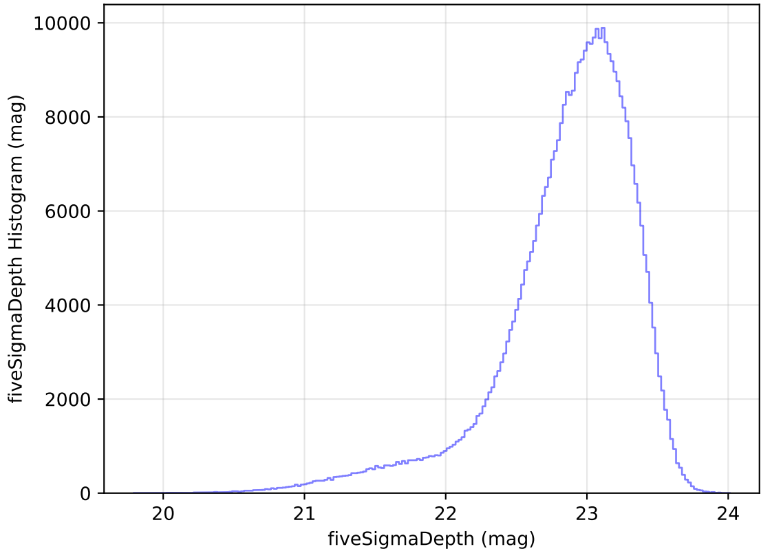
internal_u_expt38_nscale1.2v3.4_10yrs All sky z band: fiveSigmaDepth Histogram
