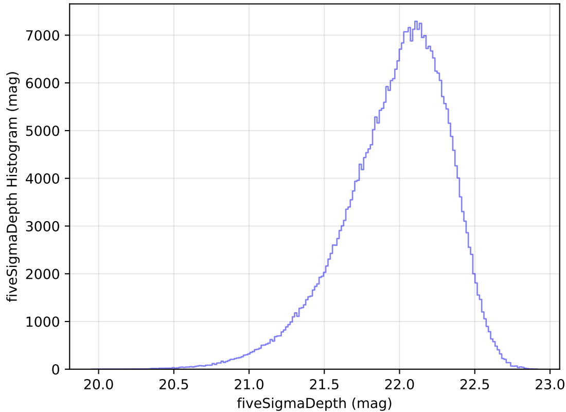
internal_u_expt38_nscale1.2v3.4_10yrs All sky y band: fiveSigmaDepth Histogram
