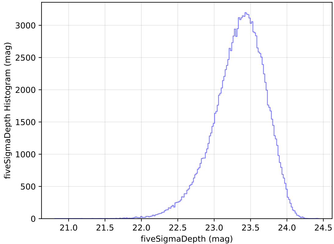
internal_u_expt38_nscale1.2v3.4_10yrs All sky u band: fiveSigmaDepth Histogram
