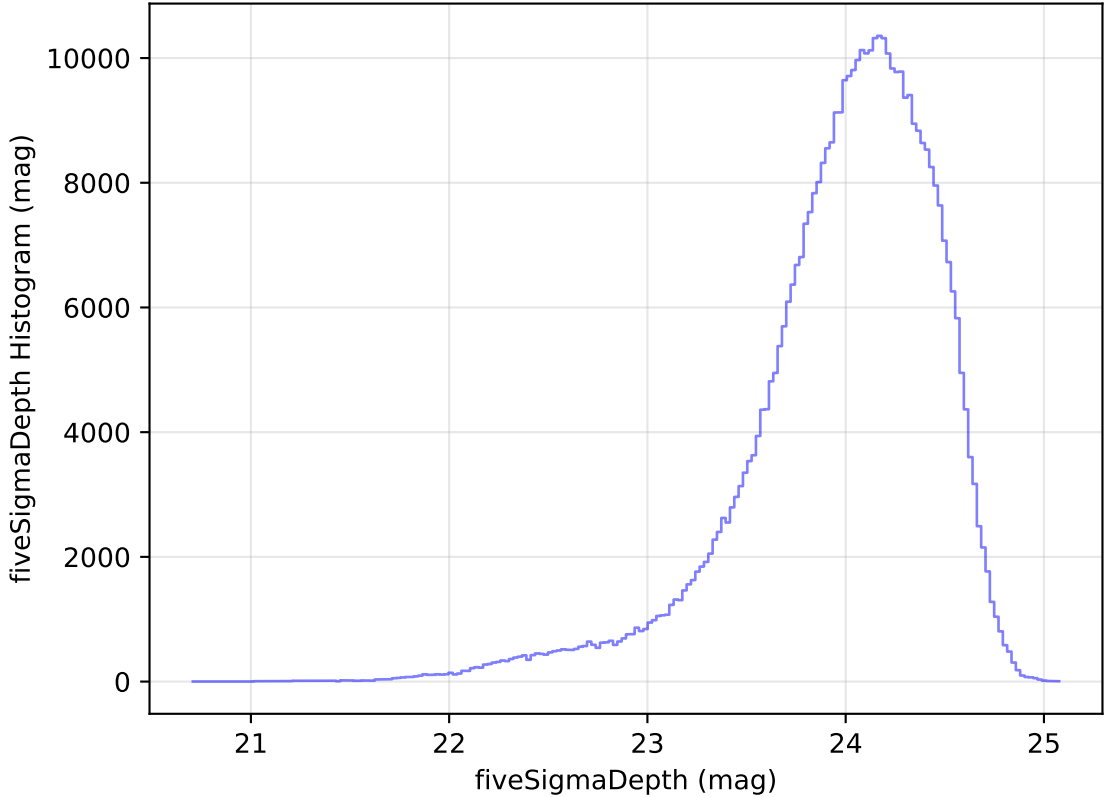
internal_u_expt38_nscale1.2v3.4_10yrs All sky r band: fiveSigmaDepth Histogram
