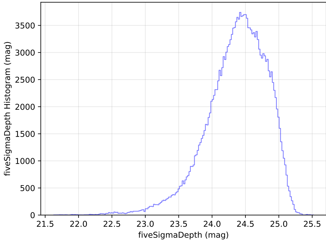
internal_u_expt38_nscale1.2v3.4_10yrs All sky g band: fiveSigmaDepth Histogram
