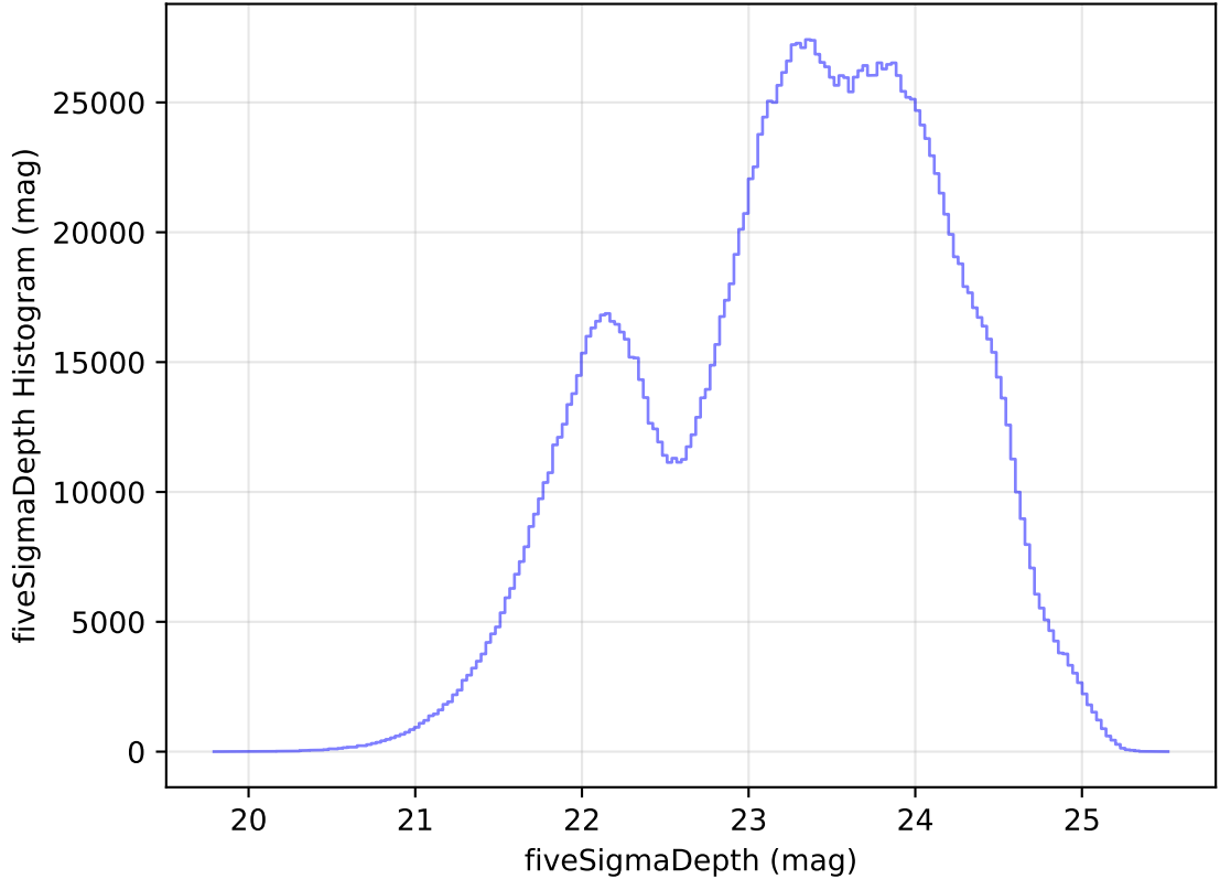
internal_u_expt38_nscale1.2v3.4_10yrs All sky all bands: fiveSigmaDepth Histogram
