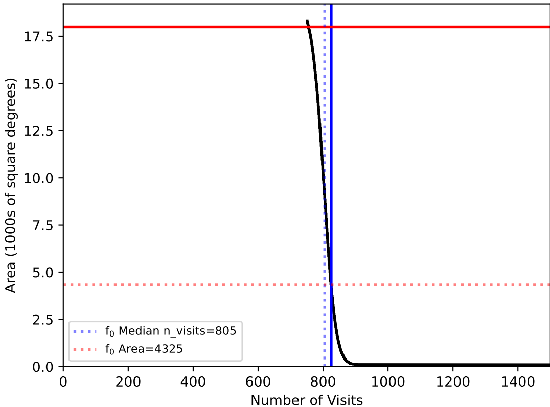
internal_u_expt38_nscale1.2v3.4_10yrs WFD: f0
