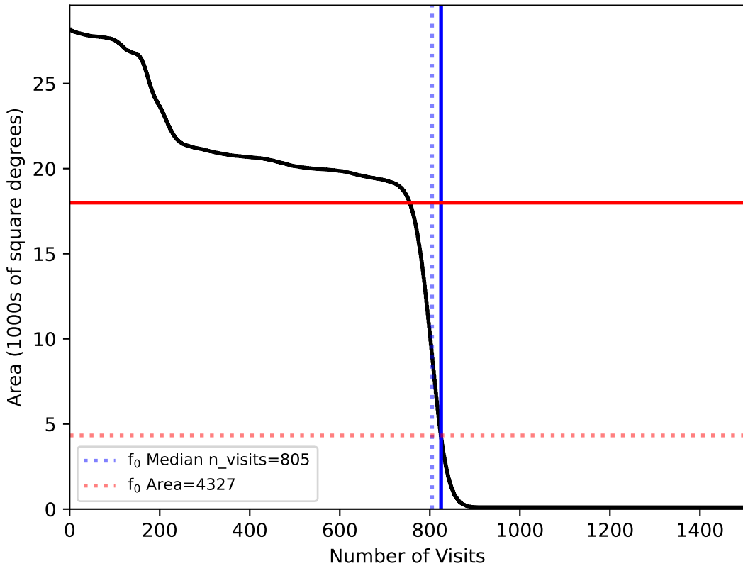
internal_u_expt38_nscale1.2v3.4_10yrs All sky: f0
