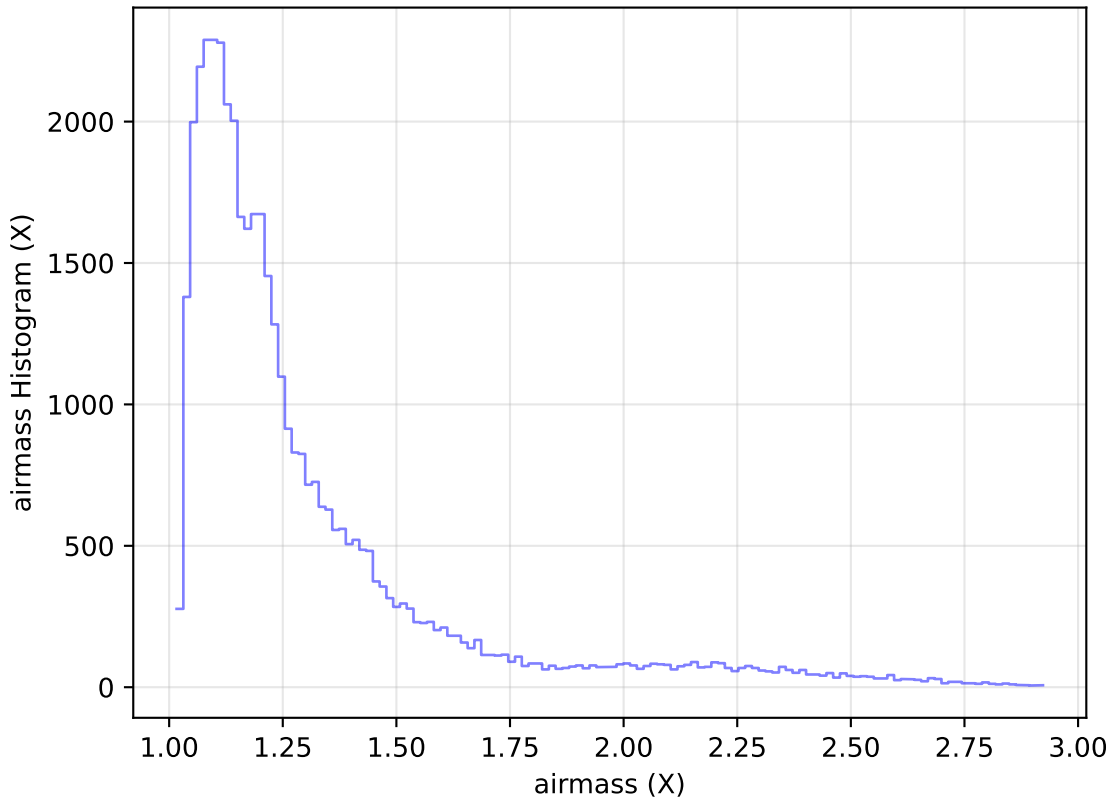
internal_u_expt38_nscale1.2v3.4_10yrs Yr 1 z band: airmass Histogram
