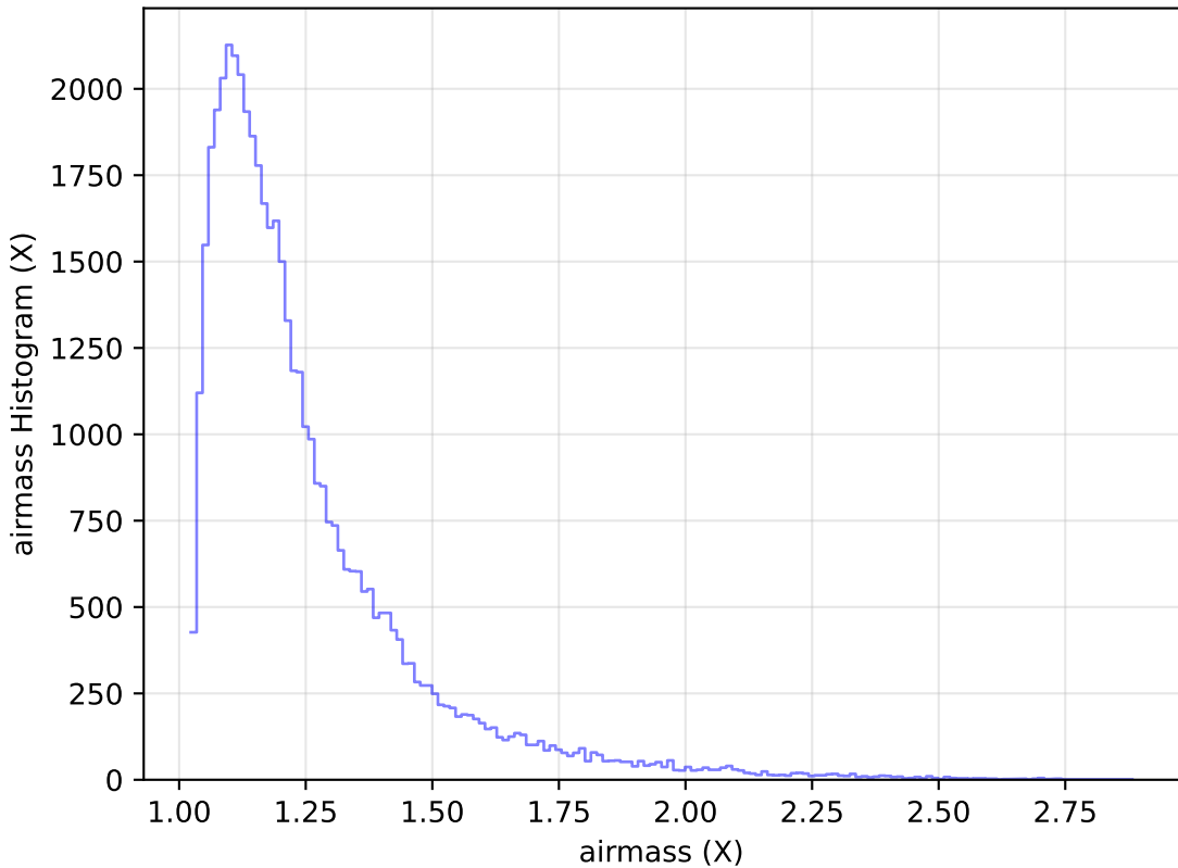
internal_u_expt38_nscale1.2v3.4_10yrs Yr 1 y band: airmass Histogram
