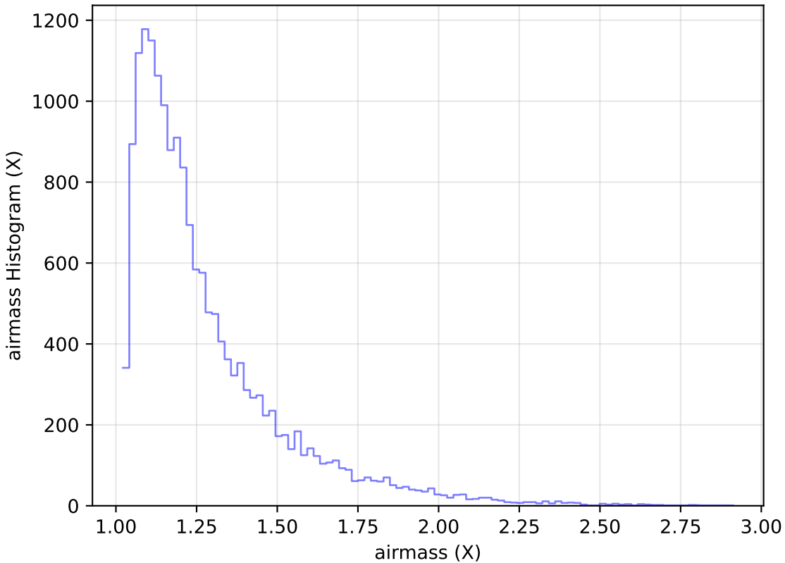
internal_u_expt38_nscale1.2v3.4_10yrs Yr 1 u band: airmass Histogram
