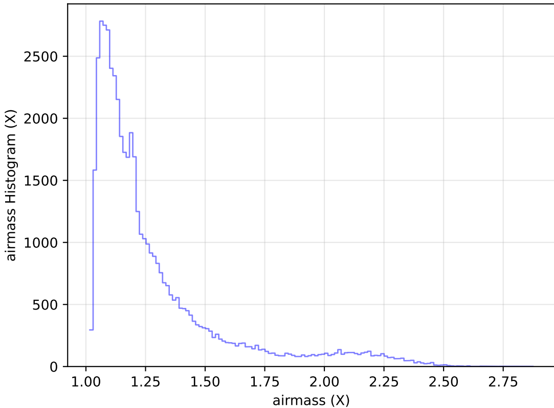
internal_u_expt38_nscale1.2v3.4_10yrs Yr 1 r band: airmass Histogram
