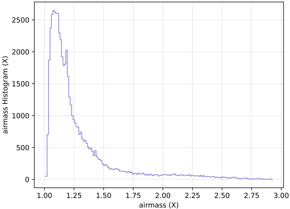
internal_u_expt38_nscale1.2v3.4_10yrs Yr 1 i band: airmass Histogram
