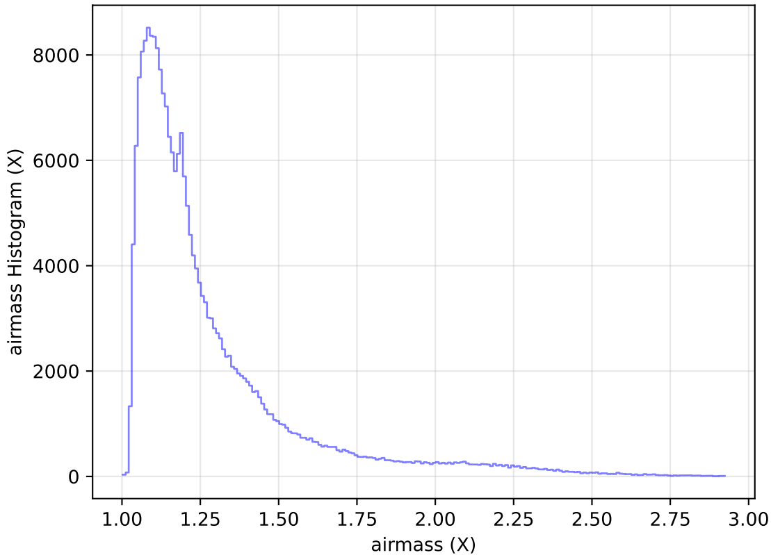
internal_u_expt38_nscale1.2v3.4_10yrs Yr 1 all bands: airmass Histogram
