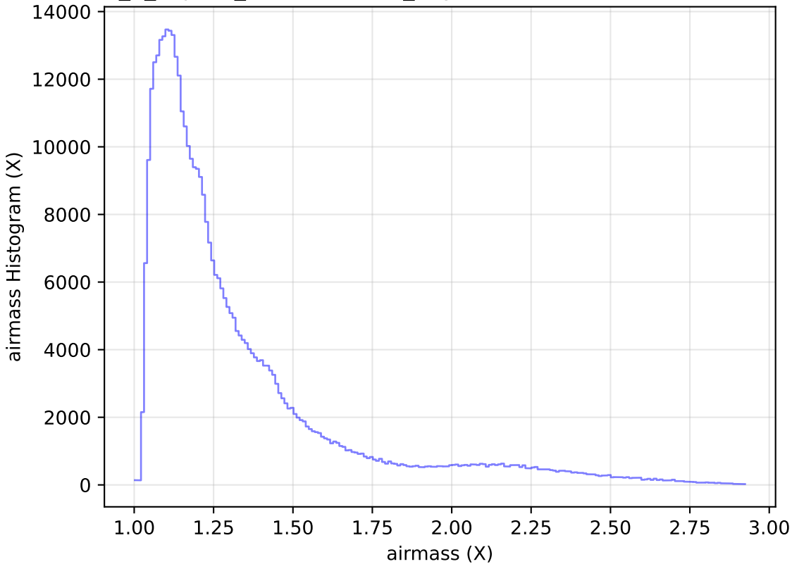
internal_u_expt38_nscale1.2v3.4_10yrs WFD z band: airmass Histogram
