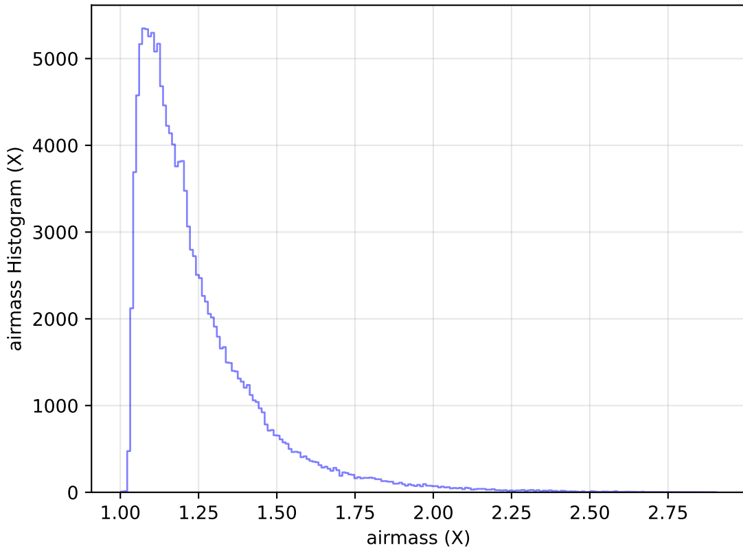
internal_u_expt38_nscale1.2v3.4_10yrs WFD u band: airmass Histogram
