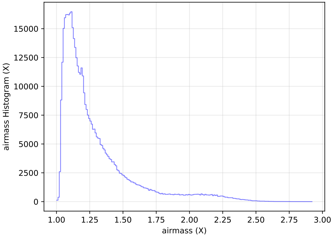
internal_u_expt38_nscale1.2v3.4_10yrs WFD r band: airmass Histogram
