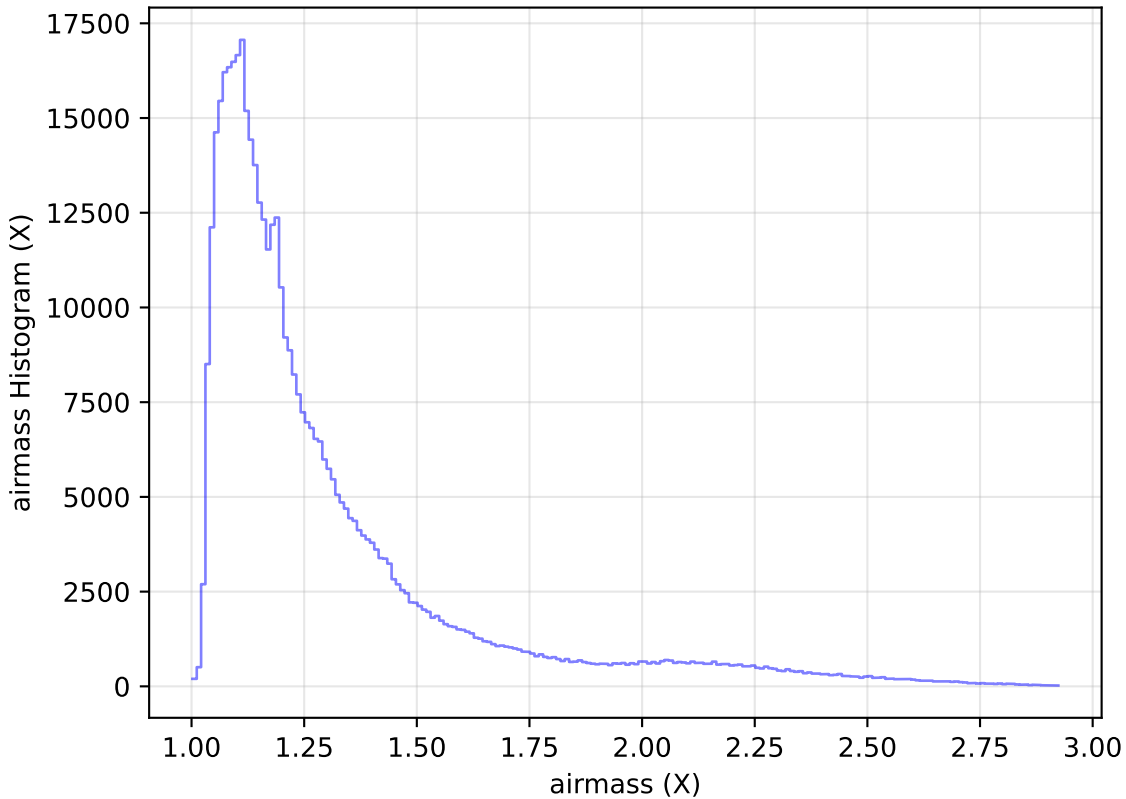
internal_u_expt38_nscale1.2v3.4_10yrs WFD i band: airmass Histogram
