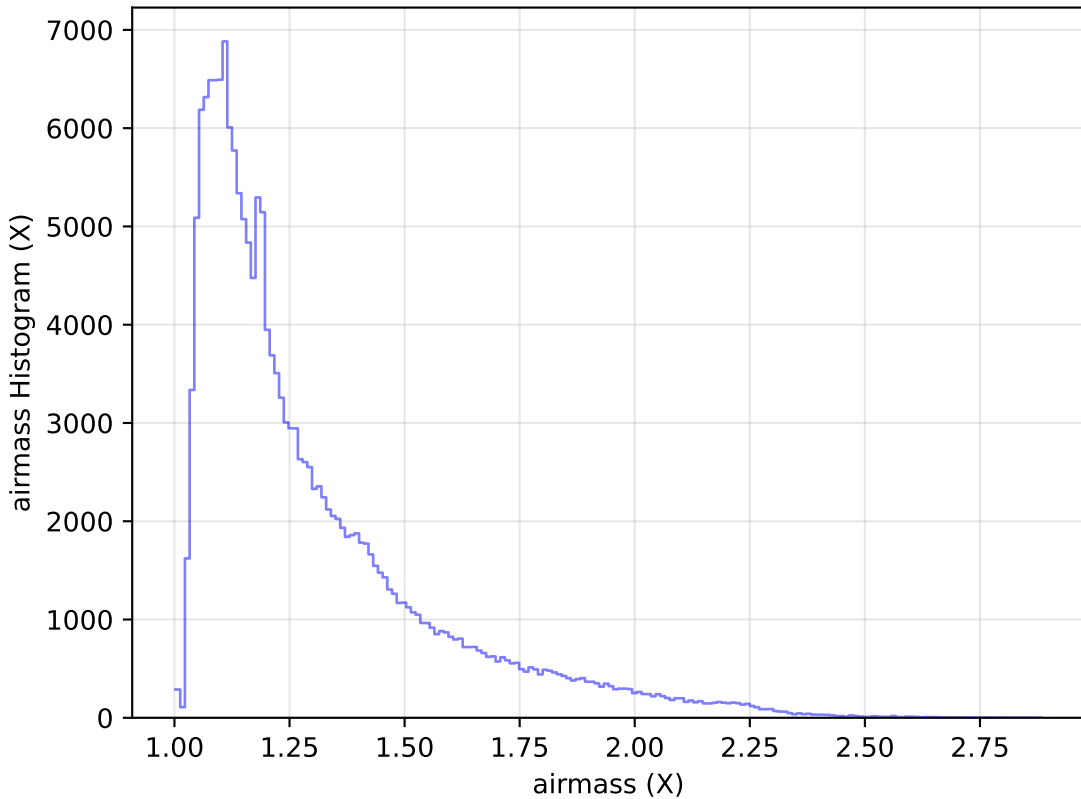
internal_u_expt38_nscale1.2v3.4_10yrs WFD g band: airmass Histogram
