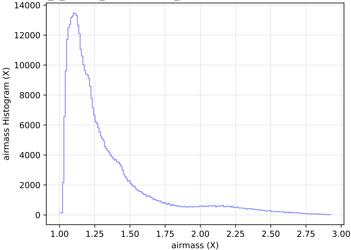
internal_u_expt38_nscale1.2v3.4_10yrs All sky z band: airmass Histogram
