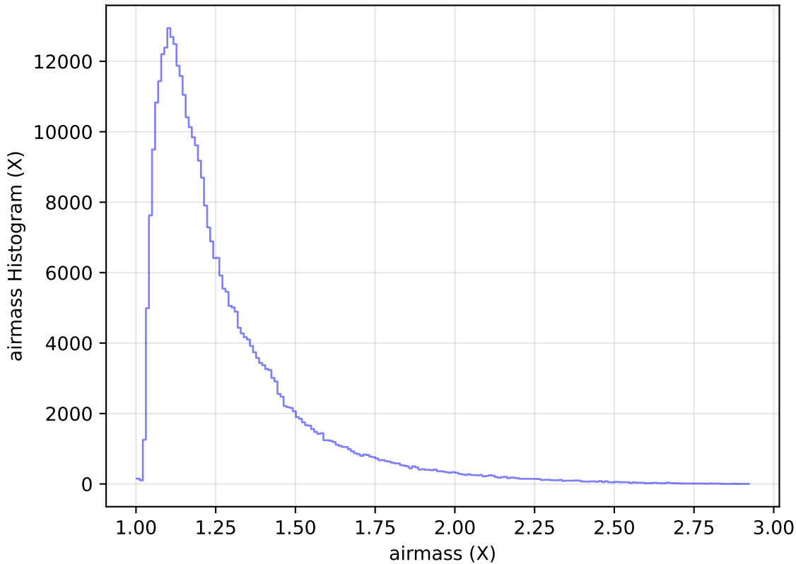
internal_u_expt38_nscale1.2v3.4_10yrs All sky y band: airmass Histogram
