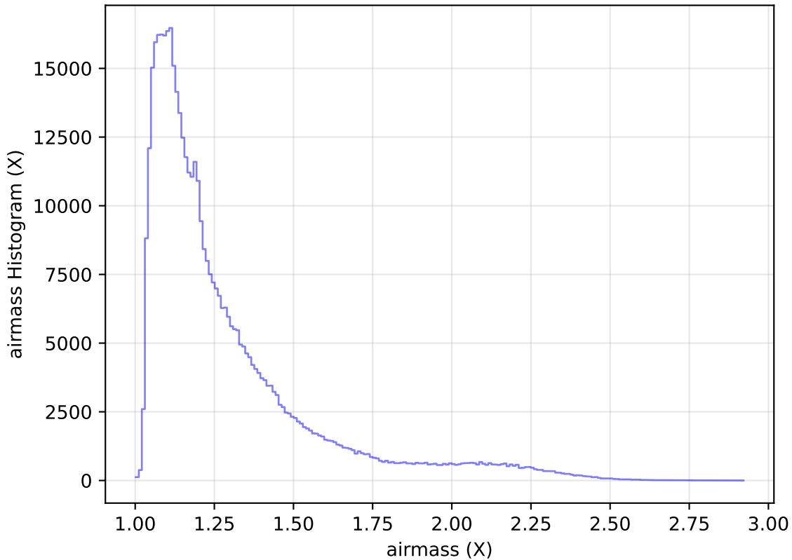
internal_u_expt38_nscale1.2v3.4_10yrs All sky r band: airmass Histogram
