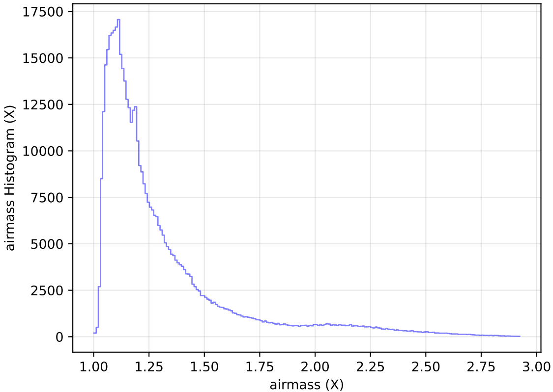
internal_u_expt38_nscale1.2v3.4_10yrs All sky i band: airmass Histogram
