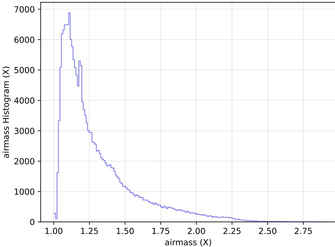
internal_u_expt38_nscale1.2v3.4_10yrs All sky g band: airmass Histogram
