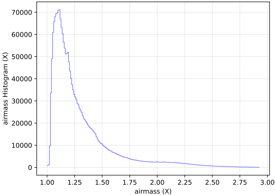
internal_u_expt38_nscale1.2v3.4_10yrs All sky all bands: airmass Histogram
