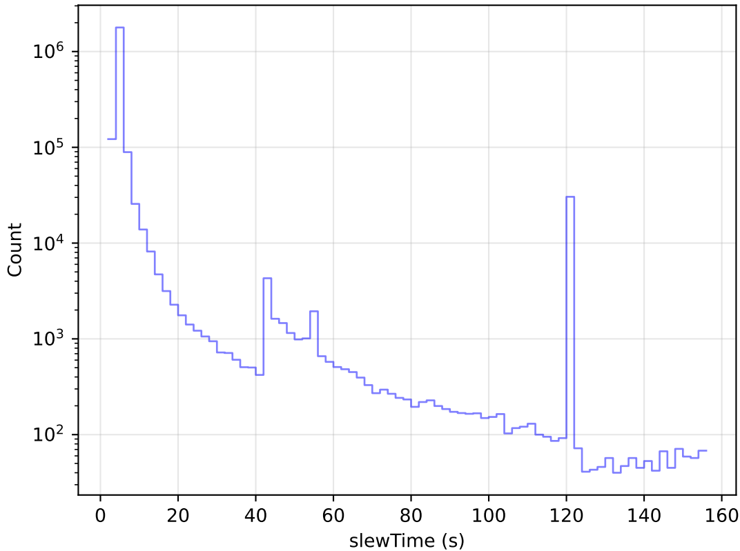
internal_u_expt38_nscale1.2v3.4_10yrs All visits: Slew Time Histogram
