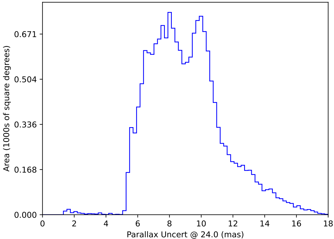
internal_u_expt38_nscale1.2v3.4_10yrs WFD: Parallax Uncert @ 24.0
