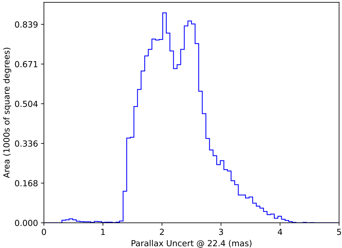
internal_u_expt38_nscale1.2v3.4_10yrs WFD: Parallax Uncert @ 22.4
