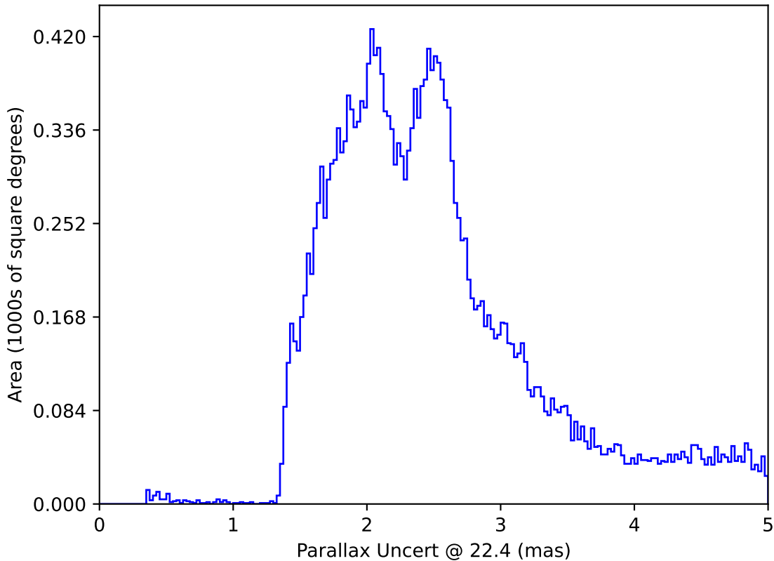
internal_u_expt38_nscale1.2v3.4_10yrs All sky: Parallax Uncert @ 22.4
