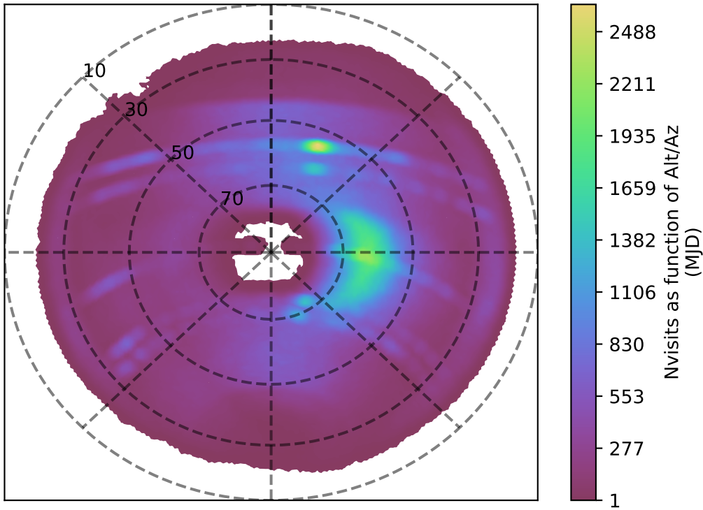
internal_u_expt38_nscale1.2v3.4_10yrs z band: Nvisits as function of Alt/Az
