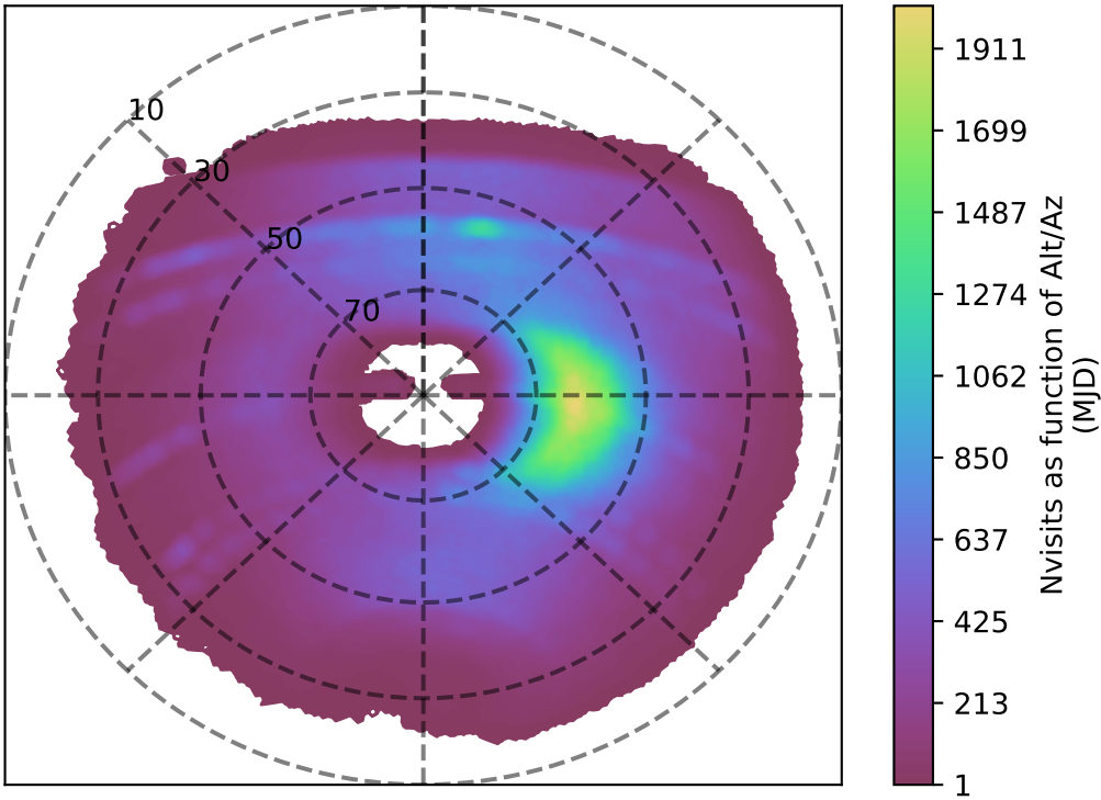
internal_u_expt38_nscale1.2v3.4_10yrs y band: Nvisits as function of Alt/Az
