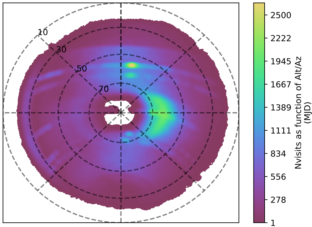
internal_u_expt38_nscale1.2v3.4_10yrs r band: Nvisits as function of Alt/Az
