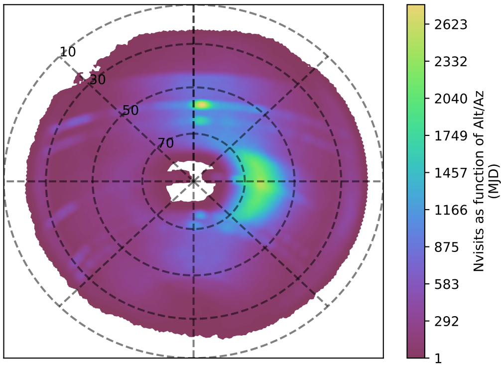
internal_u_expt38_nscale1.2v3.4_10yrs i band: Nvisits as function of Alt/Az
