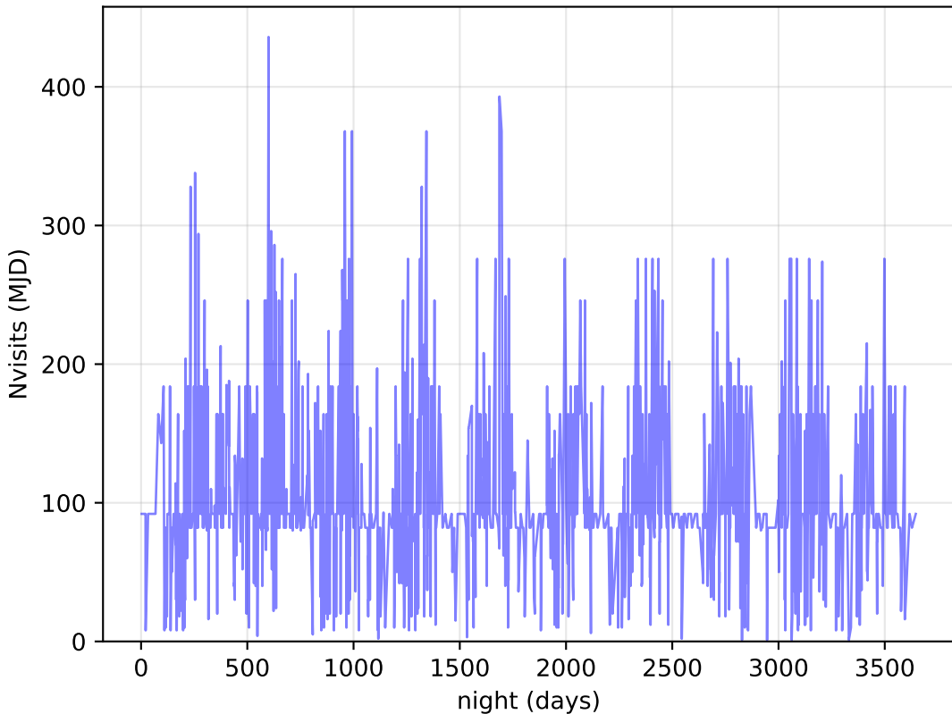
internal_u_expt38_nscale1.2v3.4_10yrs DDF: Nvisits
