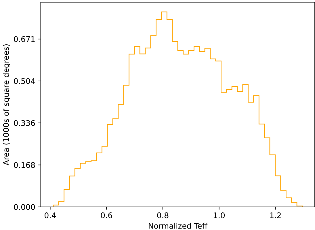
internal_u_expt38_nscale1.2v3.4_10yrs WFD r band: Normalized Teff
