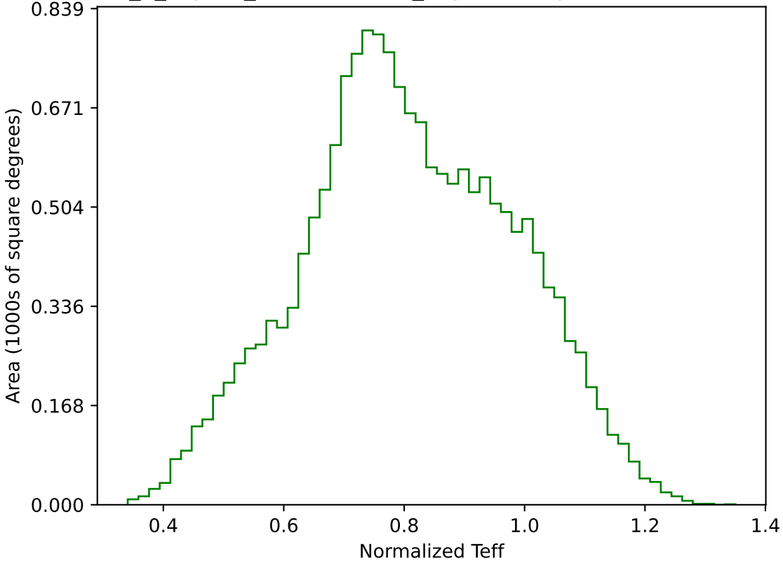
internal_u_expt38_nscale1.2v3.4_10yrs WFD g band: Normalized Teff
