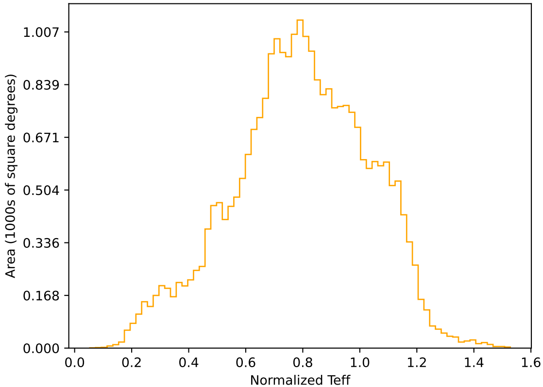
internal_u_expt38_nscale1.2v3.4_10yrs All sky r band: Normalized Teff
