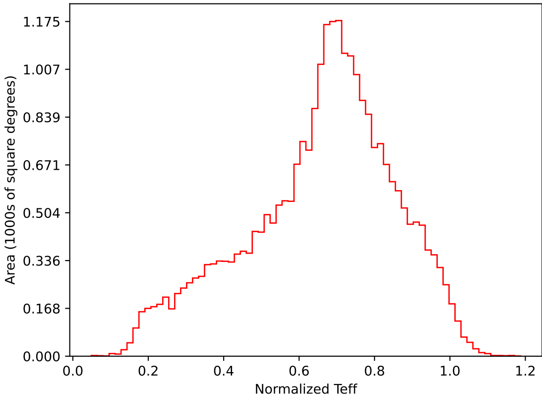
internal_u_expt38_nscale1.2v3.4_10yrs All sky i band: Normalized Teff
