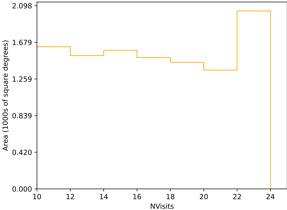
internal_u_expt38_nscale1.2v3.4_10yrs Yr 3-4 r band: NVisits
