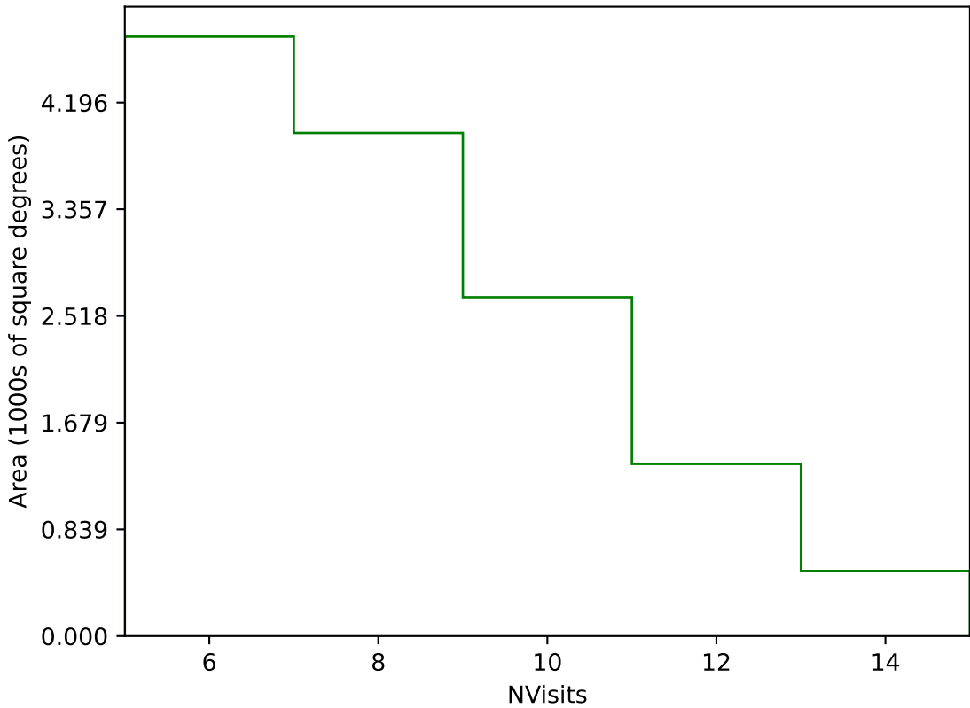
internal_u_expt38_nscale1.2v3.4_10yrs Yr 3-4 g band: NVisits
