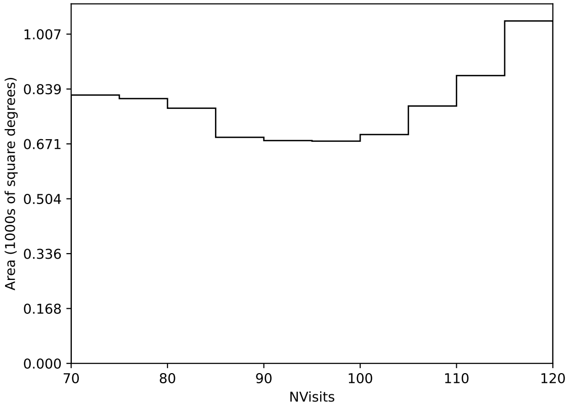
internal_u_expt38_nscale1.2v3.4_10yrs Yr 3-4 all bands: NVisits
